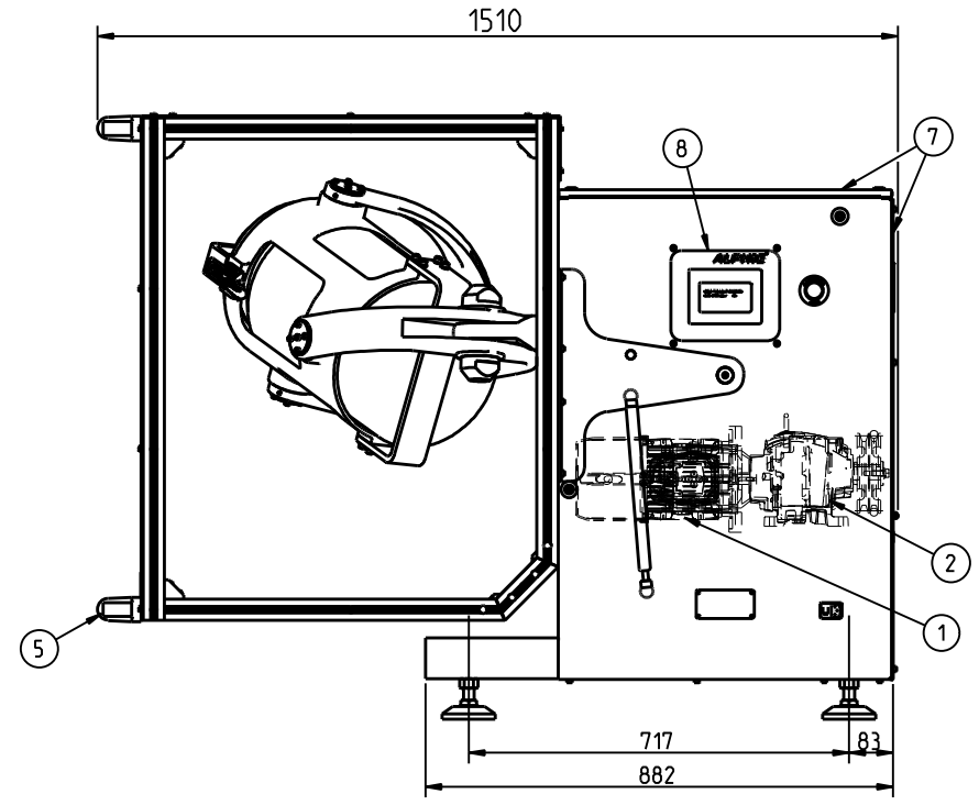
SAFETY GUARD CLOSED CONDITION
