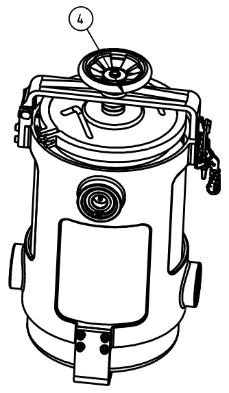
CAGE WITH CENTRE CLAMPING DEVICE
