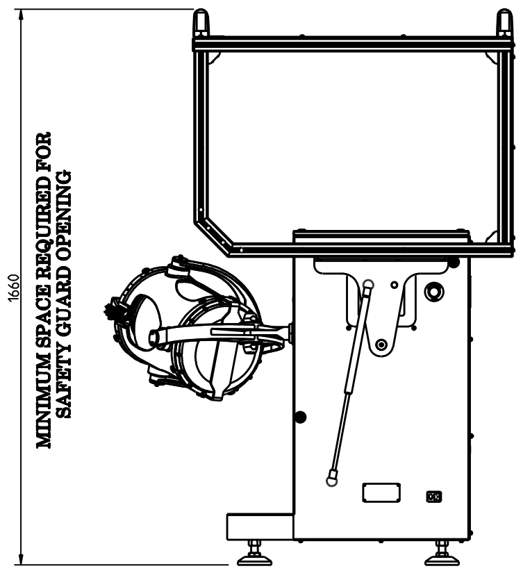
SAFETY GUARD OPENED CONDITION
