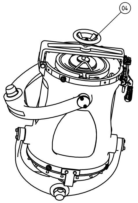
CAGE WITH CENTRE CLAMPING DEVICE
