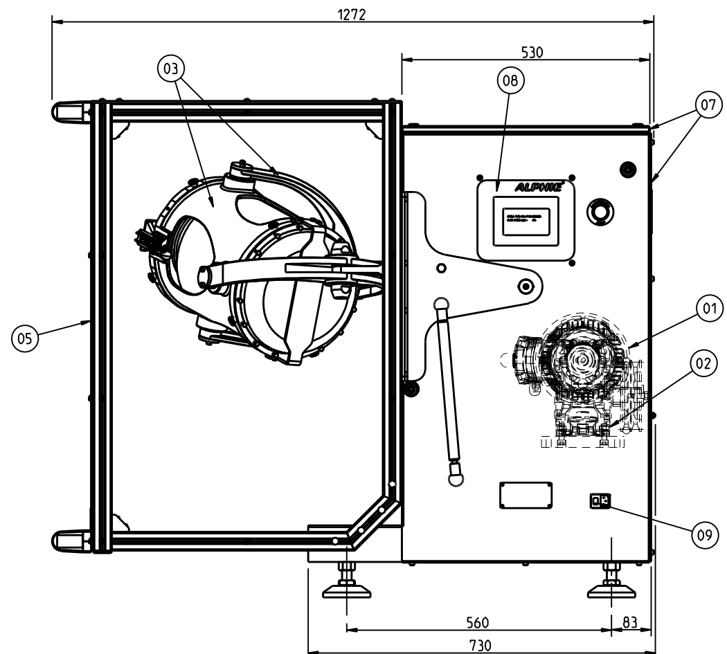
SAFETY GUARD CLOSED CONDITION
