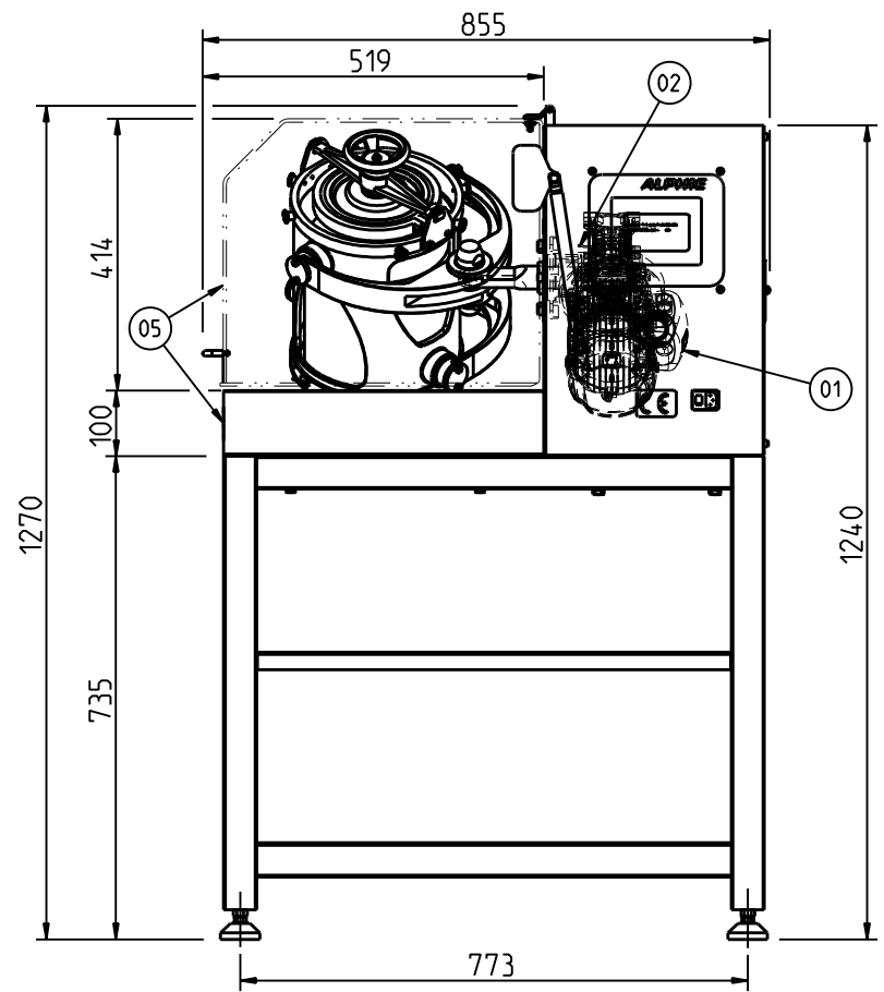
SAFETY GUARD CLOSED CONDITION
