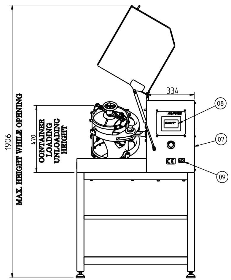
SAFETY GUARD OPENED CONDITION
