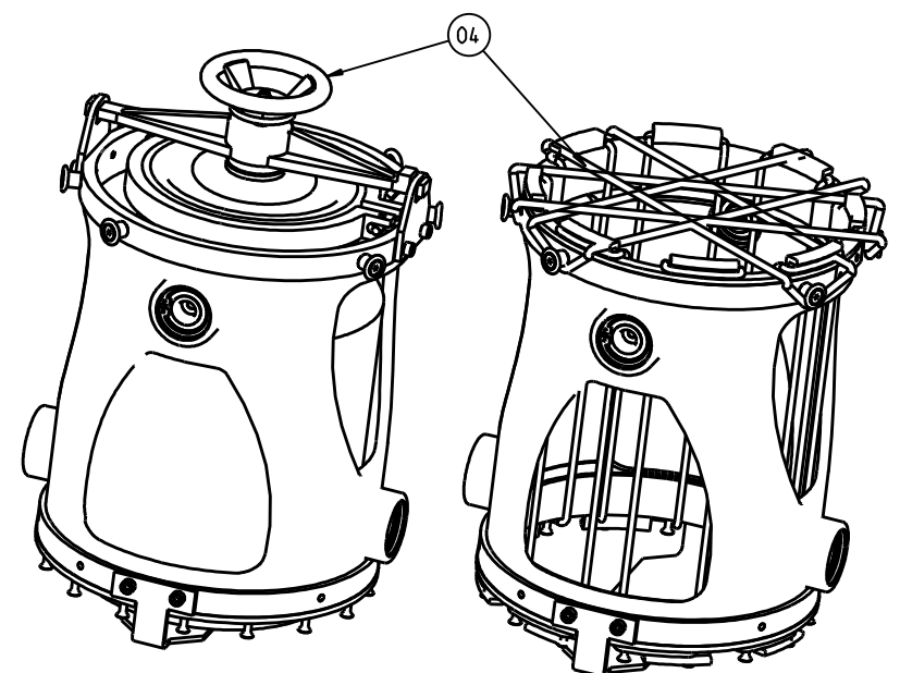
CAGE WITH CENTRE CLAMPING DEVICE CAGE WITH TENSIONING RUBBER STRING
