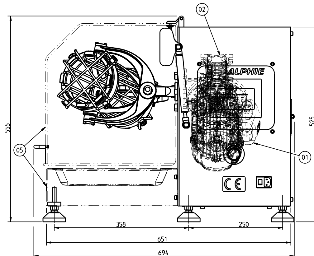
SAFETY GUARD CLOSED CONDITION
