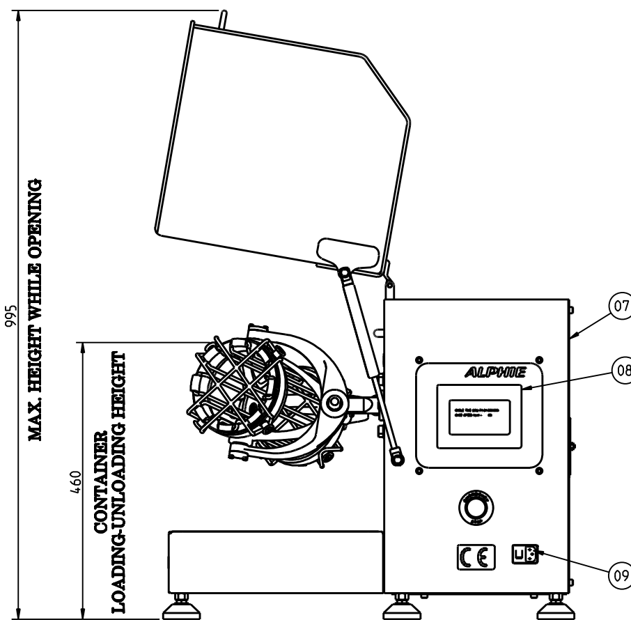
SAFETY GUARD OPENED CONDITION
